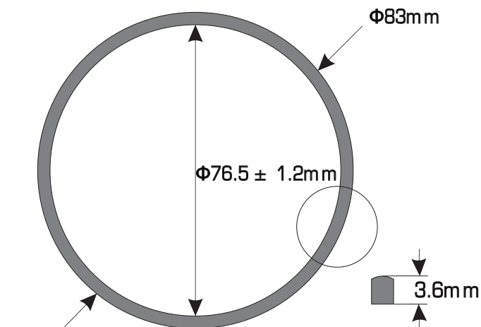
Gasket with “D”-Shaped Section
